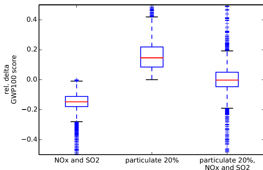
Figure 5 Effect of NO x , SO 2 and particulate on GWP100 scores
